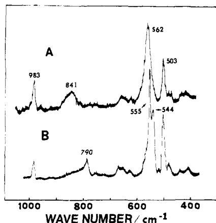
Figure 7. RR spectra of solid [\text{Co}(\text{J-en})(\text{py})_2\text{O}_2] obtained by the 587-nm excitation at \sim 150\text{K} : (A) ^{16}\text{O}_2 adduct, (B) ^{18}\text{O}_2 adduct. The 983\text{-cm}^{-1} band is due to \text{K}_2\text{SO}_4 (internal standard).
