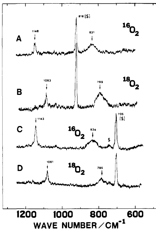
Figure 2. RR spectra of Co(J-en) in \text{CH}_3\text{CN} or \text{CH}_2\text{Cl}_2 containing 3% pyridine (580-nm excitation): (A) \text{CH}_3\text{CN} , saturated with ^{16}\text{O}_2 at -35^\circ\text{C} , (B) \text{CH}_3\text{CN} , saturated with ^{18}\text{O}_2 at -35^\circ\text{C} , (C) \text{CH}_2\text{Cl}_2 , saturated with ^{16}\text{O}_2 at -78^\circ\text{C} , and (D) \text{CH}_2\text{Cl}_2 , saturated with ^{18}\text{O}_2 at -78^\circ\text{C} . S denotes solvent bands.
