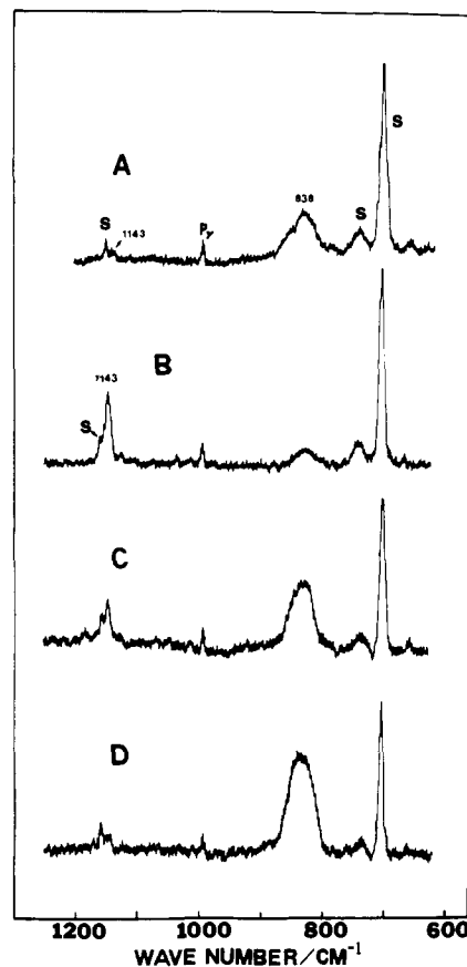
Figure 3. RR spectra of Co(J-en) in \text{CH}_2\text{Cl}_2 containing 3% pyridine which were saturated with \text{O}_2 at various \text{O}_2 pressures and temperatures (580 nm-excitation): (A) 1 atm, -78^\circ\text{C} , (B) \sim 3 atm, -80^\circ\text{C} , (C) \sim 3 atm, -30^\circ\text{C} , and (D) \sim 3 atm, +20^\circ\text{C} . S and py denote the solvent and pyridine bands, respectively.
